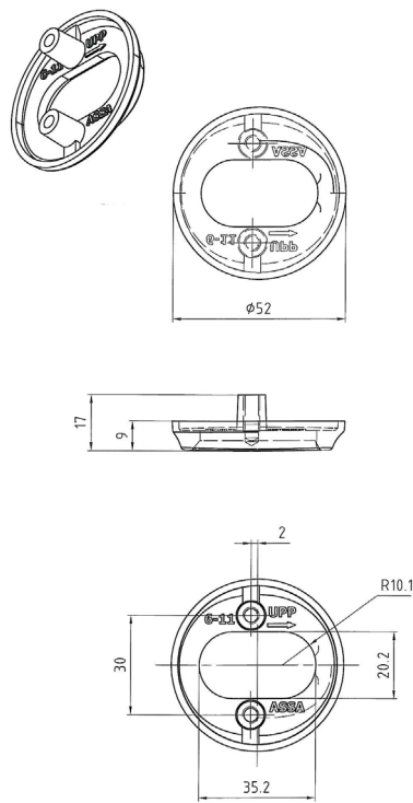
Cylinder ring, height 6-11 mm
