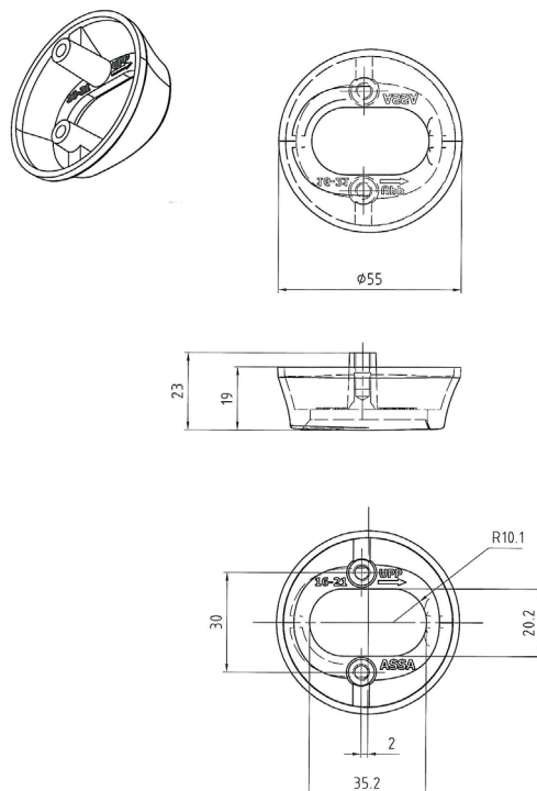
Cylinder ring, height 16-21 mm
