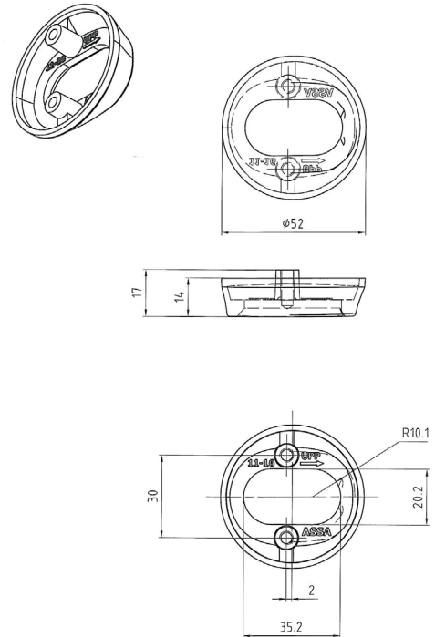
Cylinder ring, height 11-16 mm
